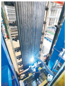
锅炉受热面INCONEL智能堆焊中心 Boiler Heating Surface INCONEL Intelligent Welding Center
